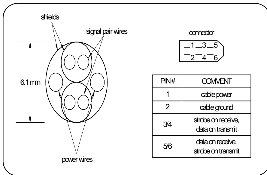
Figure 3. Cross-section of the IEEE 1394 Cable.
